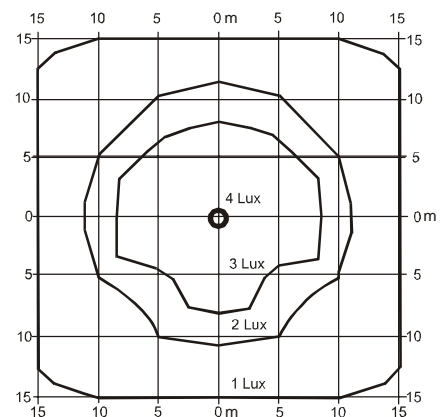
Light diagram, lamp height 4 m
